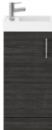
400mm Floor Standing Cabinet and Basin W400 x D222 x H781mm
